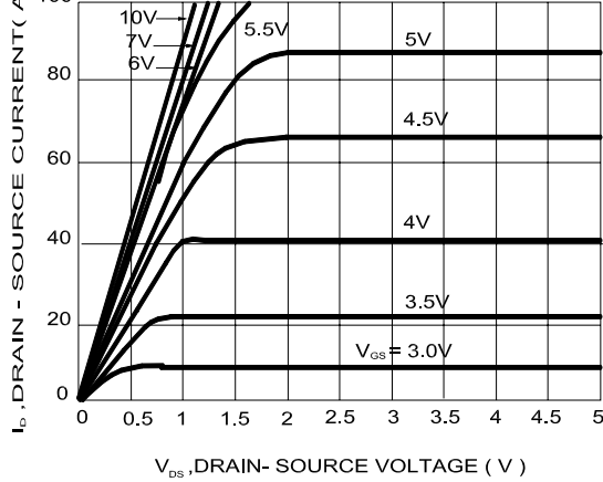
ON-REGION CHARACTERISTIC
